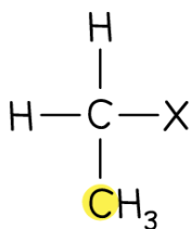
PRIMARY HALOGENOALKANE
