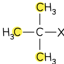
TERTIARY HALOGENOALKANE
